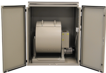
Los Angeles abrasion machine model 48-D0500/G with safety cabinet 48-D0500/CB2
